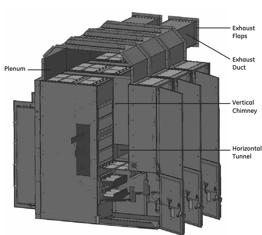
The arc resistant rear doors and plenum of a two-high design.
