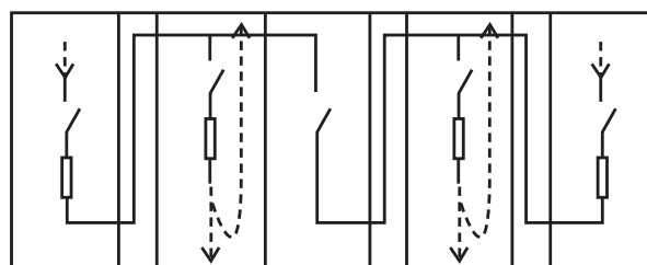
Line-up (main-tie-main)
